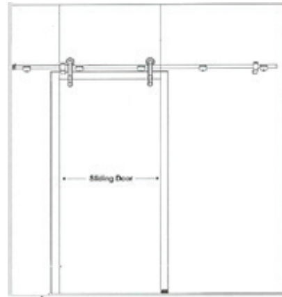
Deluxe Multihole Sliding Door System ( Max. 2 glasses )
