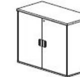
SWINGING DOOR CABINET GD 880 800W x 400D x 820H
